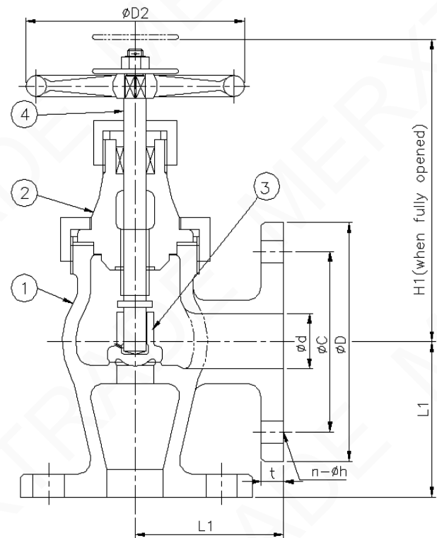
SERIES F 7412 Angle Valve
