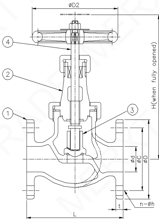
SERIES F 7411 Globe Valve
